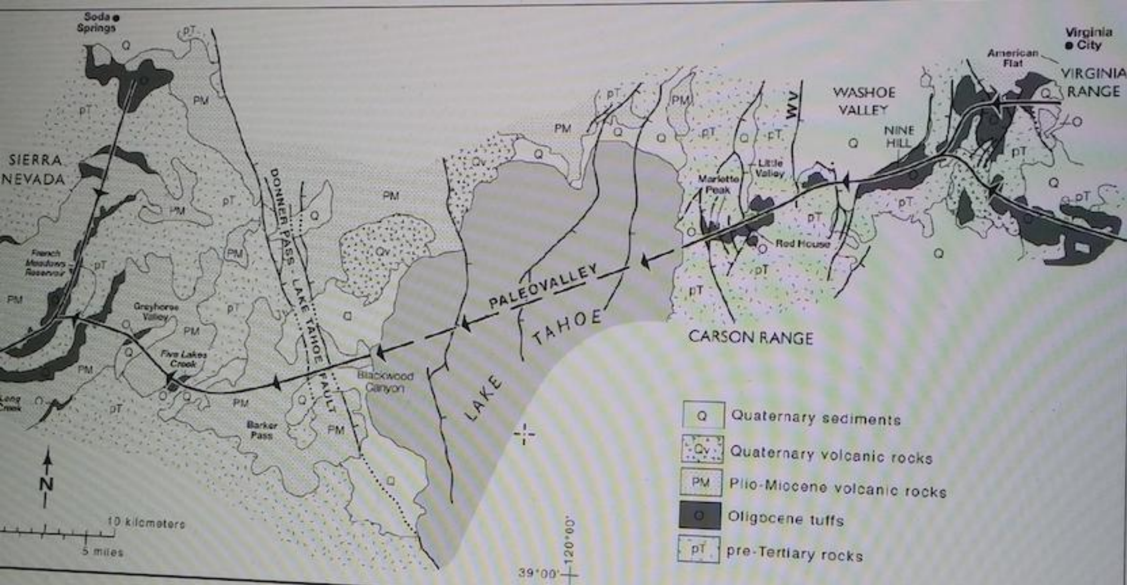
Fig. 6. Geologic map of a part of the middle Tertiary paleovalley between French Meadows and Virginia City. Contacts generalized and slightly modified from [unintelligible].
